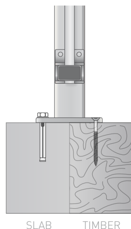
FLANGED (ON SLAB) POST DETAIL
