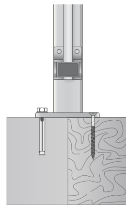
FLANGED (ON SLAB) POST DETAIL
