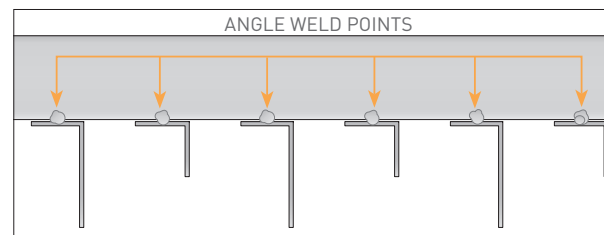
TOP ELEVATION DETAIL OF 50 X 25MM; 25 X 25MM STYLE
